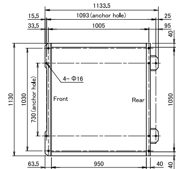
The machine installation bed channel
