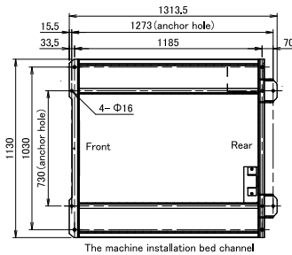
The machine installation bed channel
