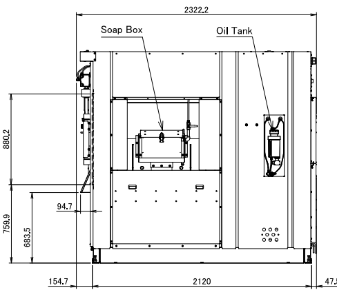
The machine installation bed channel
