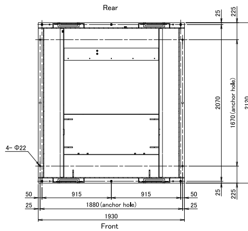
The machine installation bed channel
